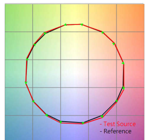
TM-30-15 Diagram
