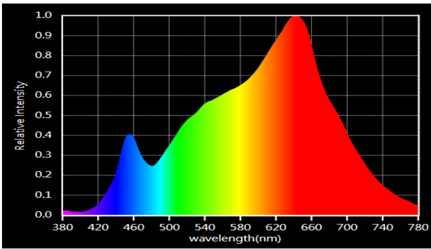
Spectral Distribution
